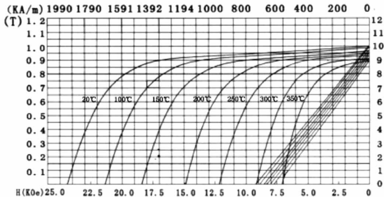
Demagnetization curves of sintered magnet SM2C017 at different temperatures
